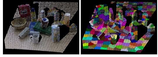
(a) The original point cloud (b) Supervoxels
